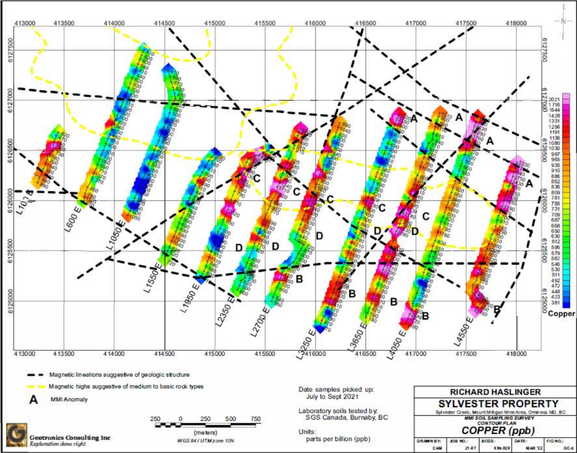
Figure 12: MMI Soil Sampling Map - Copper
