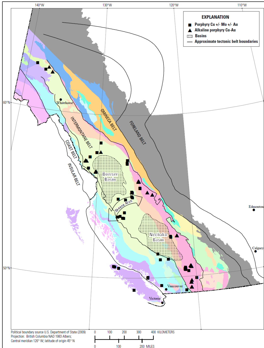
Figure 9: Distribution of porphyry copper deposits relative to generalized tectonic belts and major terranes of the Canadian Cordillera
